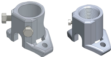
Single Band Pole Plate
