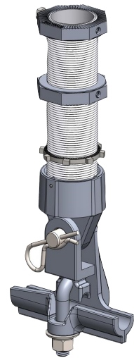
Span Wire Hanger J Bolt, Bottom Assembly
