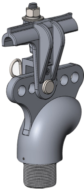
Span Wire Hanger Multi Point Top Assembly
